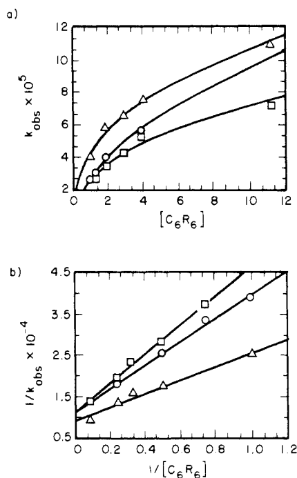
Figure 3. (a) Plot of observed rate constants versus benzene concentration: (O) reaction between 2 and C_6H_6 , ( \square ) 2 and C_6D_6 , ( \Delta ) 2-d 6 and C_6D_6 . (b) Inverse plot: symbols denote the same reactions as in plot 5a .
